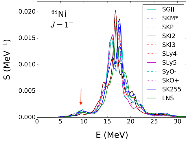
FIG. 1. Strength function for the E1 RPA response in ^{68}\text{Ni} calculated with formalism described in Ref. [22]. The calculation is performed for several Skyrme interactions, shown in the figure inset. The arrow shows the location of the pygmy resonance.
