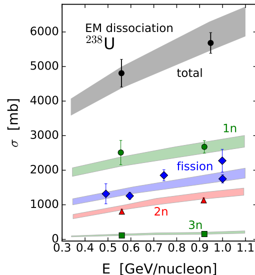
FIG. 3: Cross-section for EM dissociation of {}^{238}\text{U} . The excited nucleus decays by fissioning (diamonds) and multiple neutron emission ( xn ) [39–42]. Theoretical calculations and their uncertainty bands are also shown [37].
