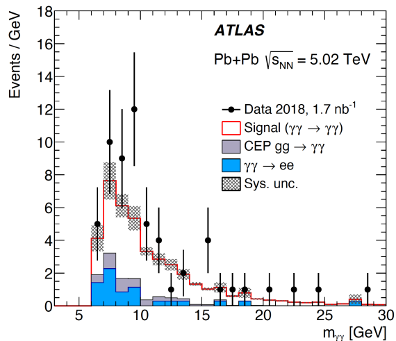
FIG. 11: Number of light-by-light scattering events observed with the ATLAS detector [101].
