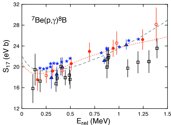
FIG. 2: Radiative capture reaction {}^7\text{Be}(p,\gamma){}^8\text{B} . The dashed line is the no-core shell-model calculation of Ref. [21] and the dotted line is from the resonant group method calculation of Ref. [23]. Experimental data are from Refs. [24–31].
