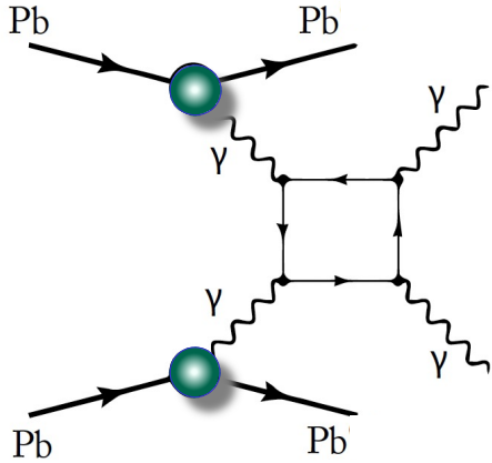
FIG. 10: Light-by-light scattering using UPCs.
