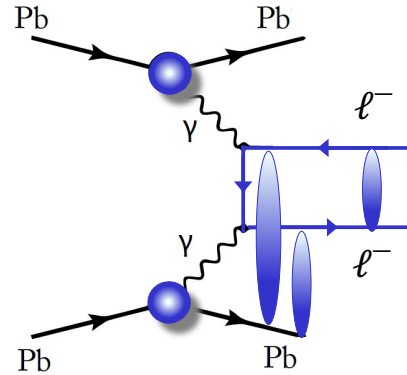
FIG. 5: Production of lepton-antilepton in UPCs. Higher-order processes, including the production of multiple pairs, might be important.
