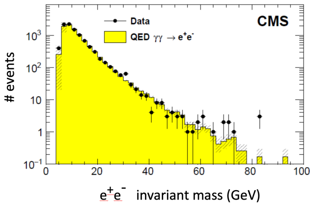
FIG. 6: e^+e^- pairs produced in UPCs observed with the CMS detector (from Ref. [66]).
