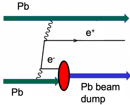
FIG. 7: Pair production with electron capture leading to possible beam losses [7].
