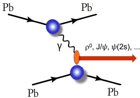
FIG. 12: Production of vector mesons in UPCs.
