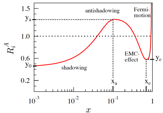
FIG. 13: Medium modification function displaying various effects as the momentum fraction x varies.
