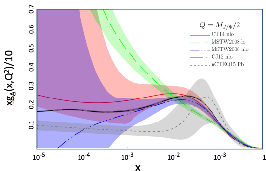
FIG. 15: Uncertainties in theoretical compilations of gluon distribution functions as a function of the momentum fraction x .
