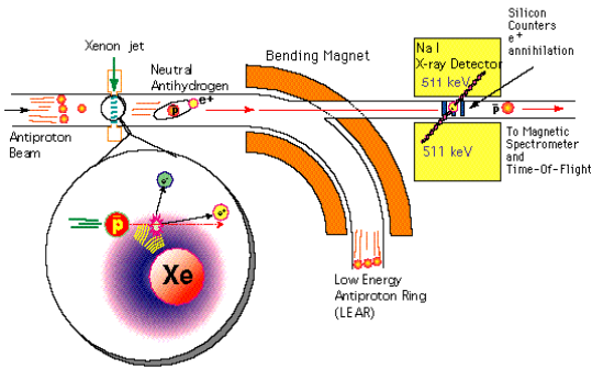
FIG. 8: Experimental setup employed in the identification of anti-atoms at the LEAR/CERN in 1996.
