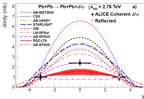
FIG. 14: Production of J/\Psi in UPCs at the LHC as a function of the rapidity y . It serves as a probe of different PDFs (adapted from Ref. [124]).
