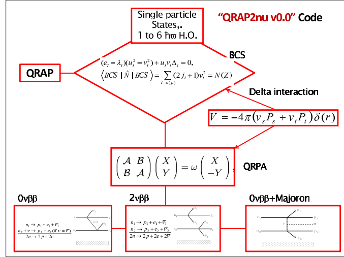
FIGURE 3. Flux diagram for QRAP-2 \nu v0.0 code.
