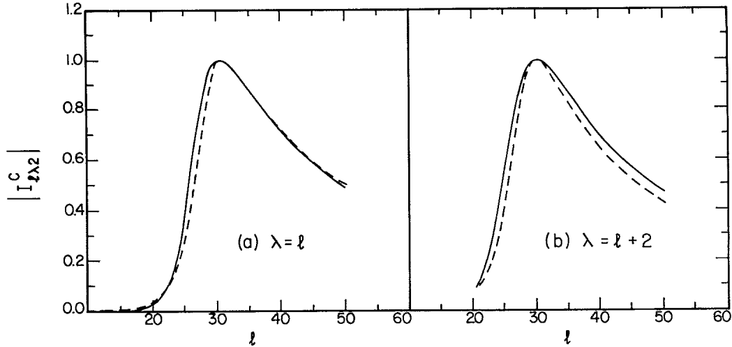
FIG. 2. The Coulomb radial integral for L=2 vs l . Solid curve is the exact result obtained from the radial wave functions, Eq. (16). The dashed curve represents Eq. (26). See text for details.
