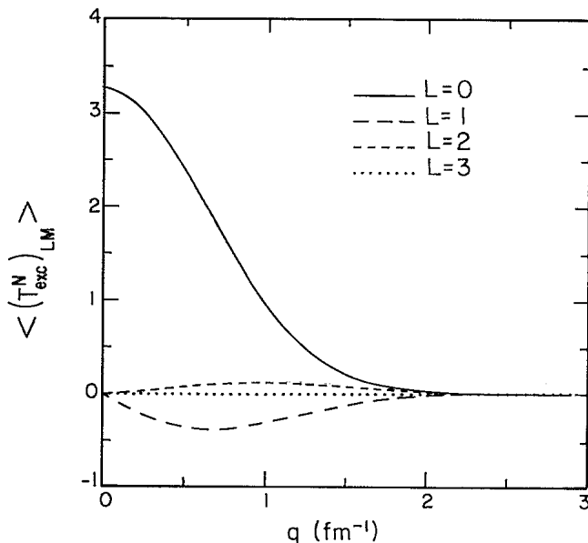
FIG. 1. The excitation T matrix, T_{\text{exc}}^N(q) , Eq. (9) for L=0 , L=1 , L=2 , and L=3 for the system ^{16}\text{O} + ^{28}\text{Si} \rightarrow \alpha + ^{12}\text{C} + ^{28}\text{Si} , at 4A MeV. The optical potential used is a typical strong absorption potential (see Ref. [1]).
