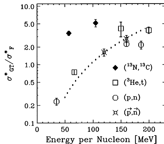
FIG. 4. Energy dependence of \sigma_{GT}^*/\sigma_F^* for a number of charge-exchange reactions performed on 13 C targets. The dotted line is the equivalent of the \hat{\sigma}_{GT}/\hat{\sigma}_F = [E_p/(55 \text{ MeV})]^2 curve, scaled appropriately.
