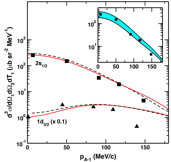
Figure 2: (Color online) Cross sections for ^{40}\text{Ca}(p,2p)^{39}\text{K} with incident proton energy E_p = 148 MeV, as a function of the recoil momentum, p_{A-1} of the residual nucleus. The proton knockout is assumed to be either from the 1d_{3/2} or from the 2s_{1/2} orbital in ^{40}\text{Ca} . The cross sections are integrated over the energy of the knocked-out proton and given in units of \mu\text{b sr}^{-2} \text{MeV}^{-1} . The experimental data are taken from Ref. [17]. The dashed (solid) lines include (do not include) the spin-orbit part of the optical potential. The inset panel shows that larger uncertainties arise, e.g., for the 1s_{1/2} state, with the inclusion of various nucleon-nucleon (NN) interactions. The shaded area contains a broad range of results obtained with different NN-interactions taken from Refs. [21, 23, 30–34].
